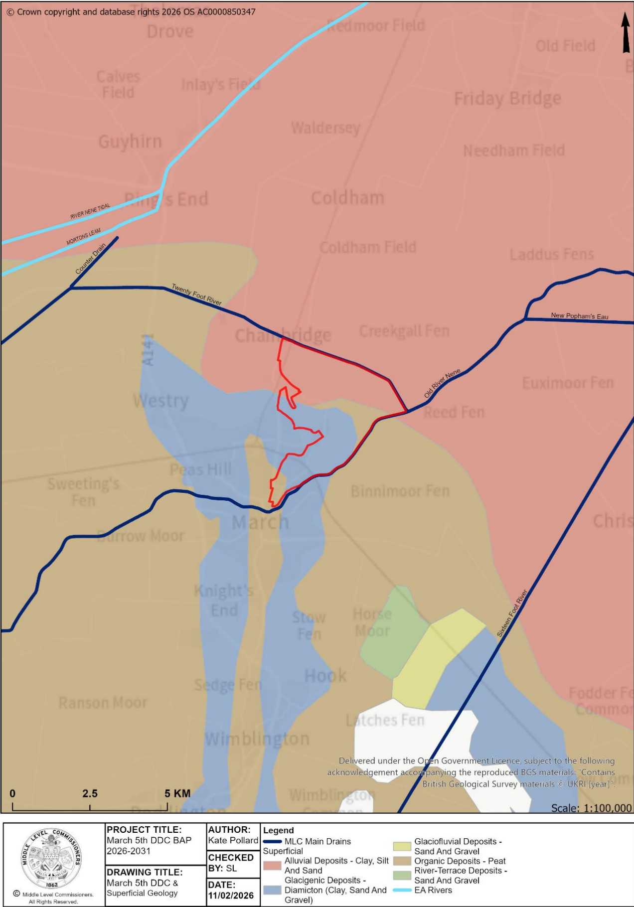
Figure 2. March 5th DDC map of superficial geology
