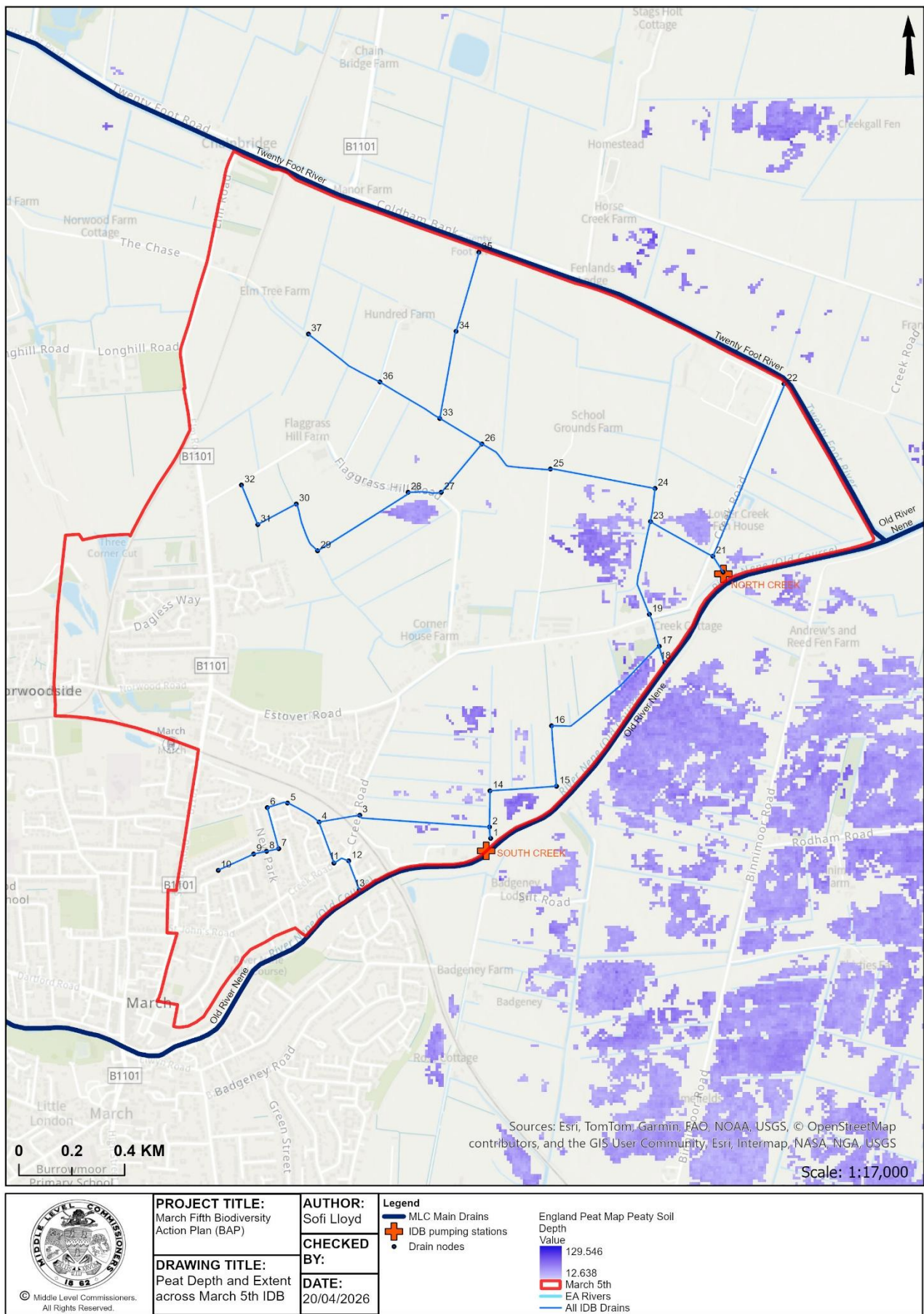
Figure 4 - Peat Depths across March 5th DDC area
