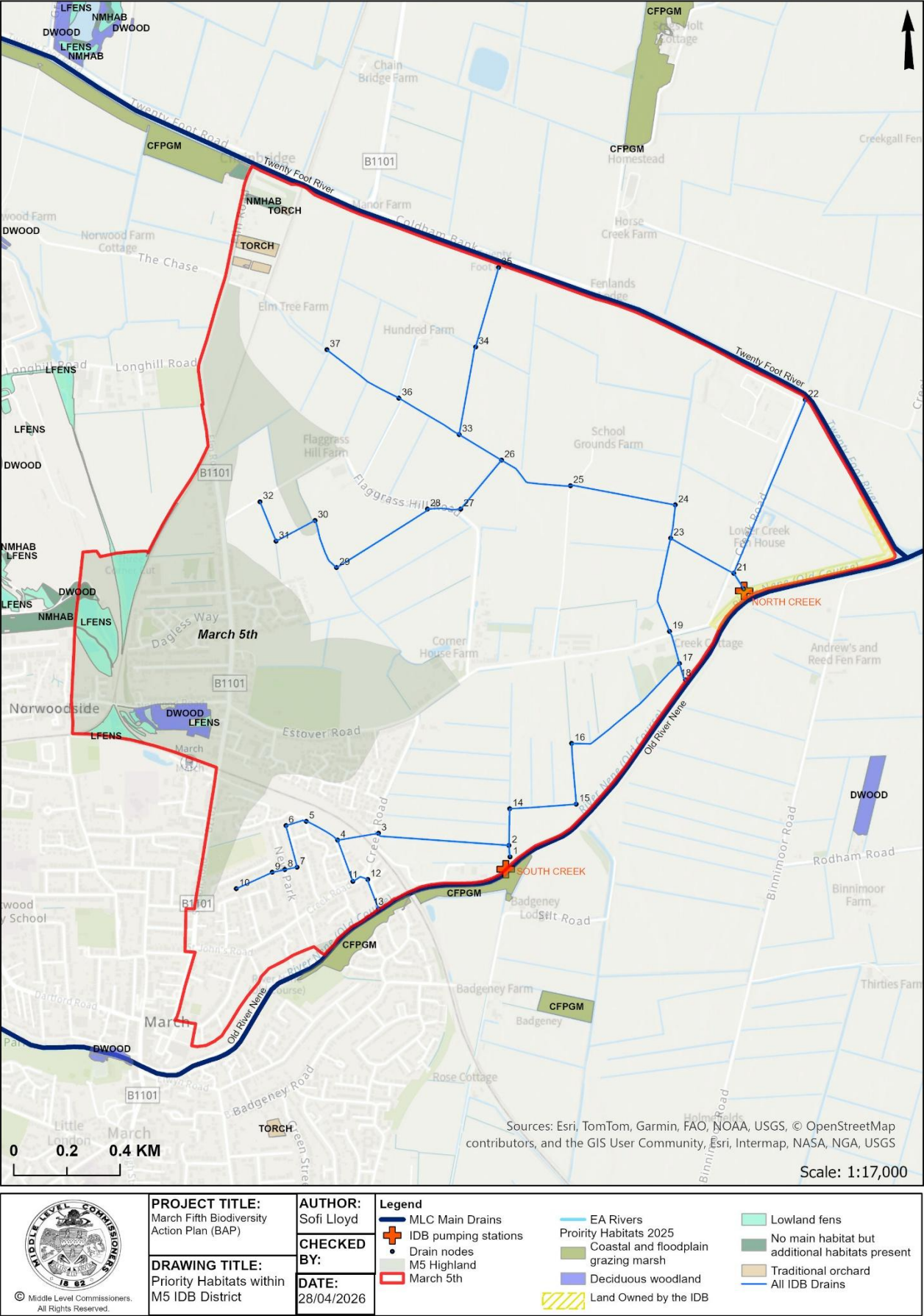
Figure 8. Map of Priority Habitats in March 5th District Drainage Commissioners Area
