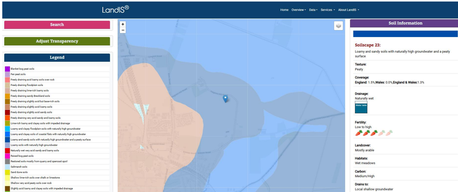
Figure 3. March 5th DDC map of soils
