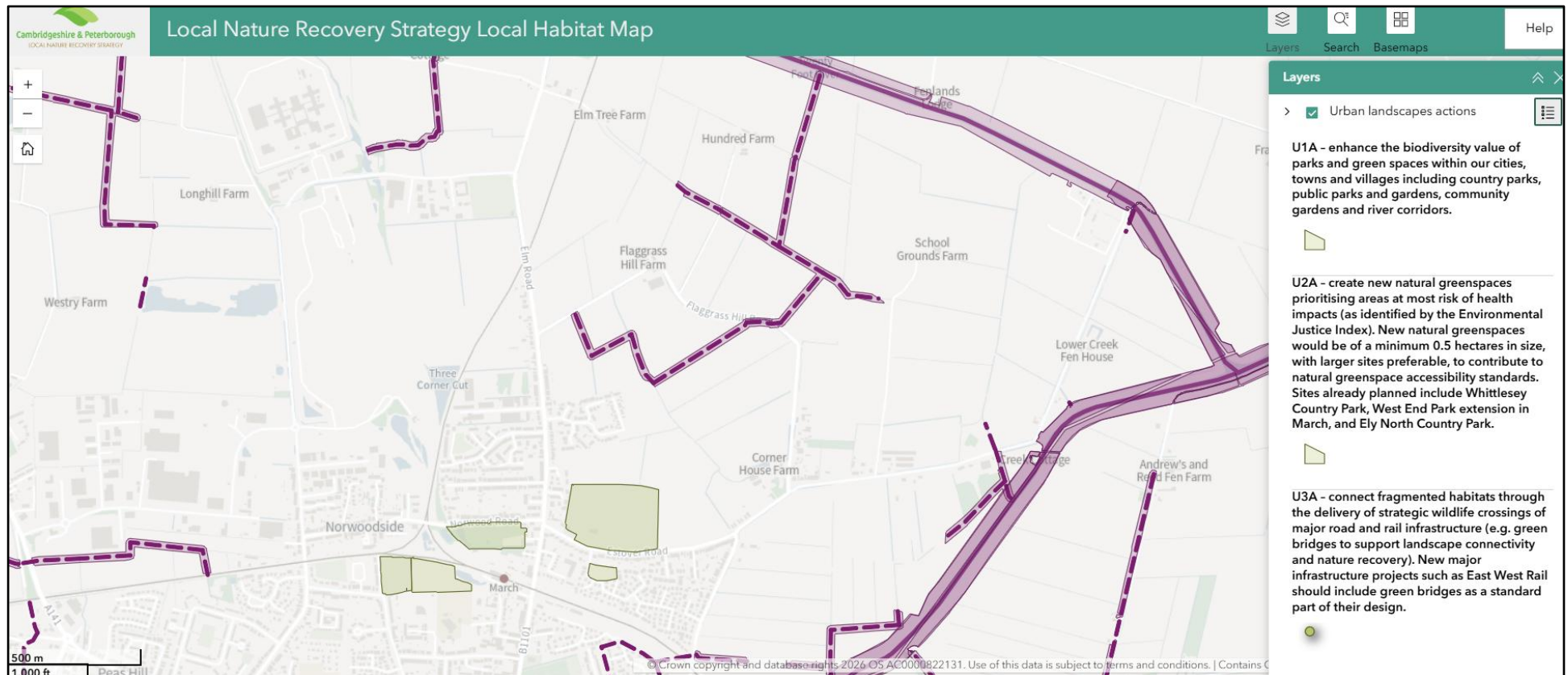
Figure 9. Mapped Priority Habitat Action Opportunities as detailed in the Cambridgeshire LNRS (published: 23 rd December 2025) in March 5th District Drainage Commissioners, available from this link: https://www.cambridgeshire.gov.uk/residents/climate-change-energy-and-environment/improving-the-natural-environment/cambridgeshire-and-peterborough-local-nature-recovery-strategy#local-nature-recovery-strategy-published-5-0
