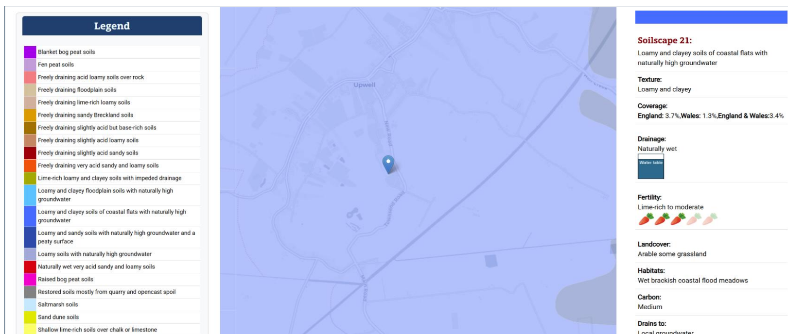
Figure 3. Churchfield and Plawfield IDB map of soil types showing a predominantly “Loamy and clayey soils of coastal flats with naturally high groundwater”
