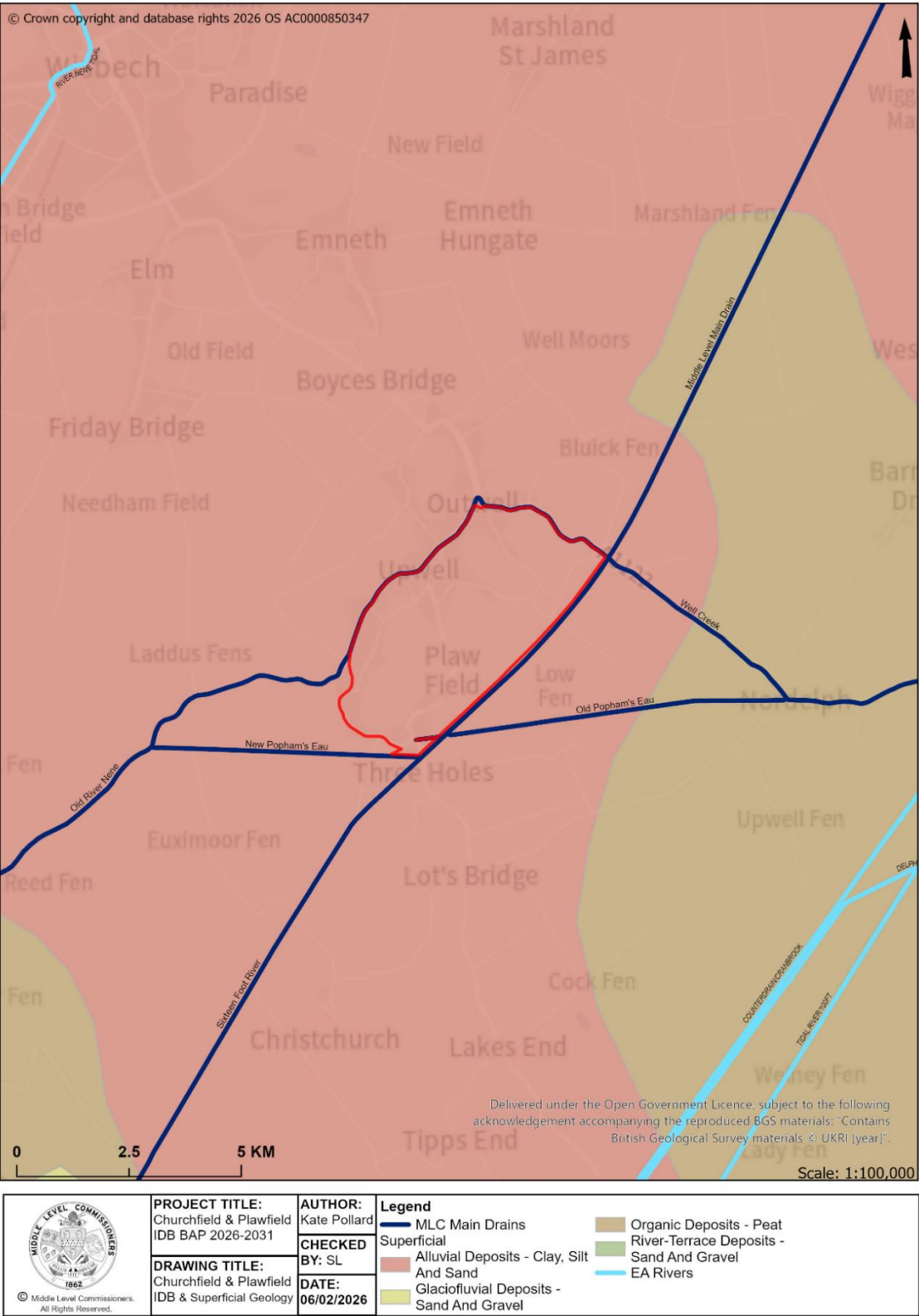
Figure 2. Churchfield and Plawfield IDB map of superficial geology
