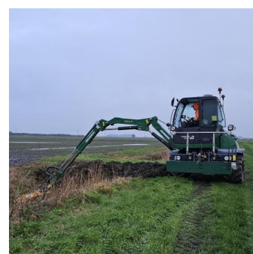
Blocked culvert, reach 83-84
